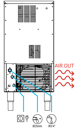
REAR VIEW
